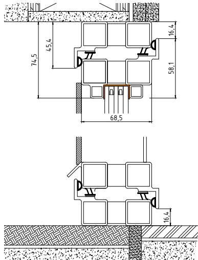
VERTICAL SECTION
