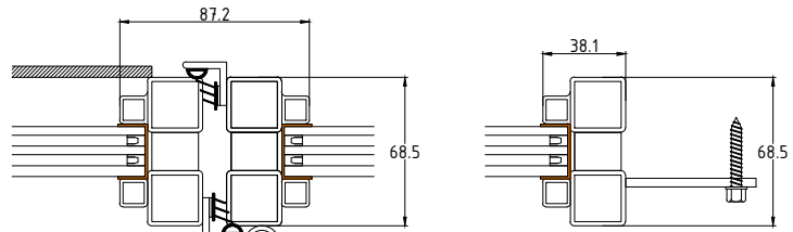
HORIZONTAL SECTION
