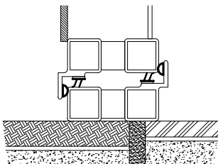
VERTICAL SECTION
