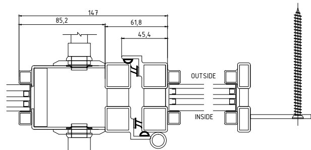
JAMB & LOCK BOX HORIZONTAL SECTION
