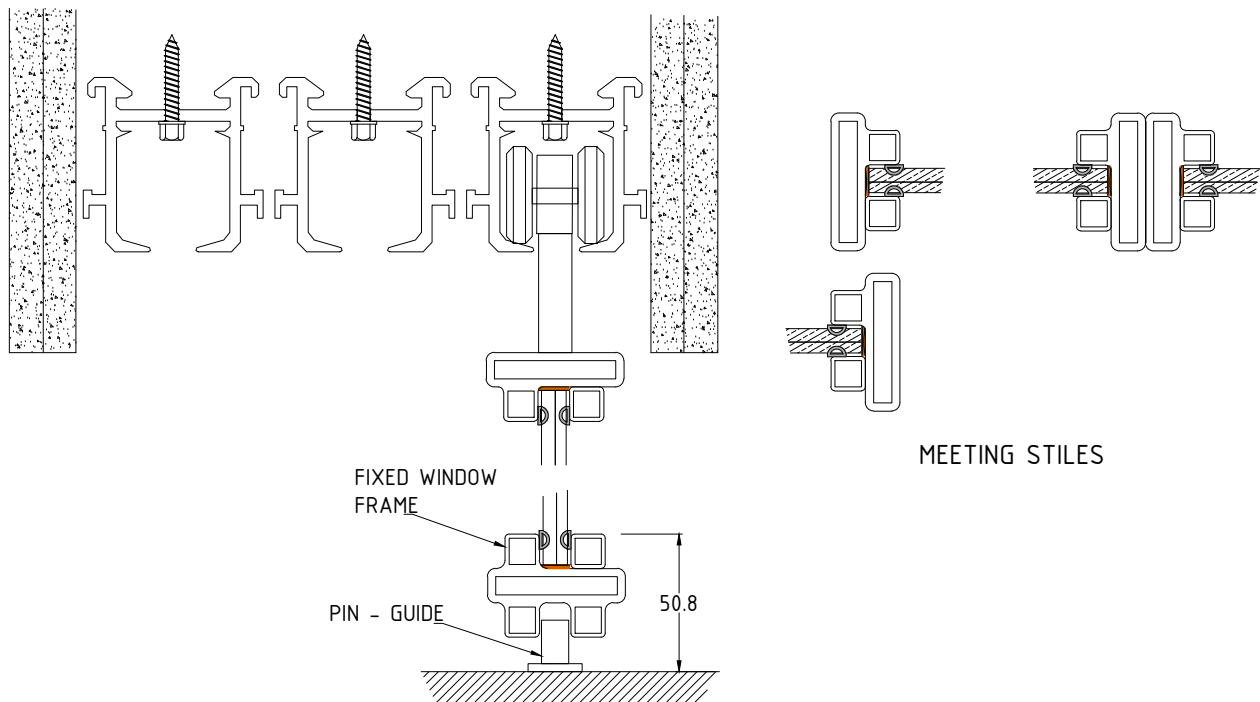
VERTICAL SECTION
