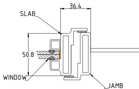
HORIZONTAL SECTION
