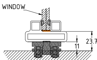
VERTICAL SECTION
